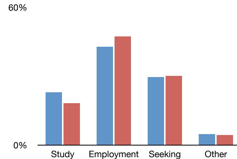
Health
