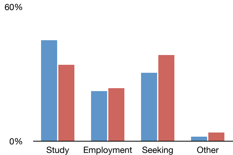
Chemistry
