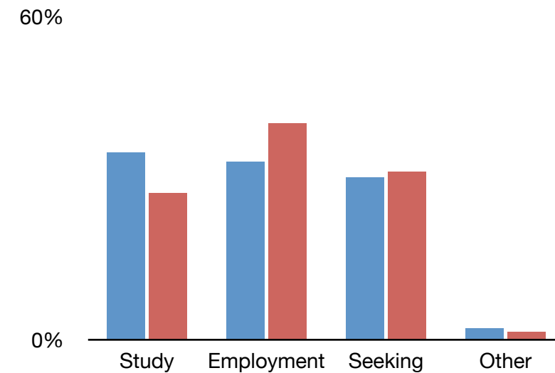
Math
